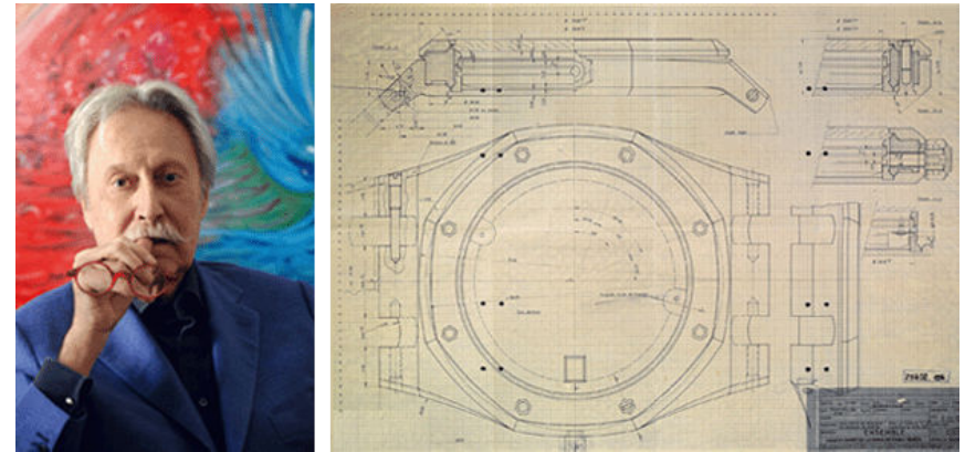
Left: Gerald Genta. Image: Audemars Piguet Archive. Right: Technical drawing of the Royal Oak Ref. 5402. Image: Audemars Piguet Archive
